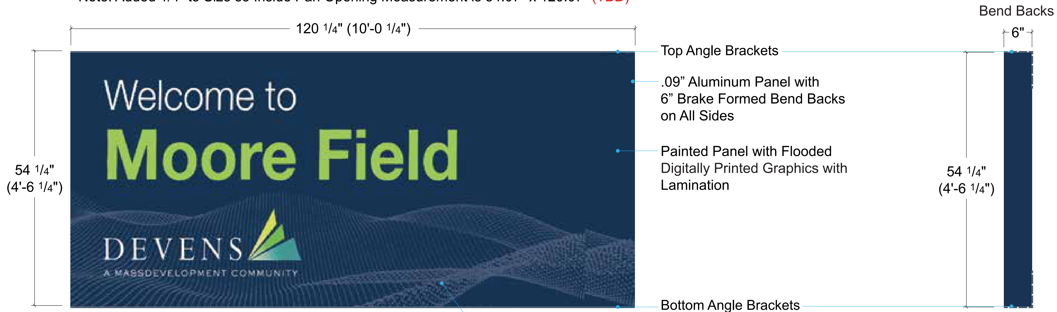
E1 Elevation: (Qty-1) #13626 Aluminum Pane Overlay Scale: 1/2"=1'
